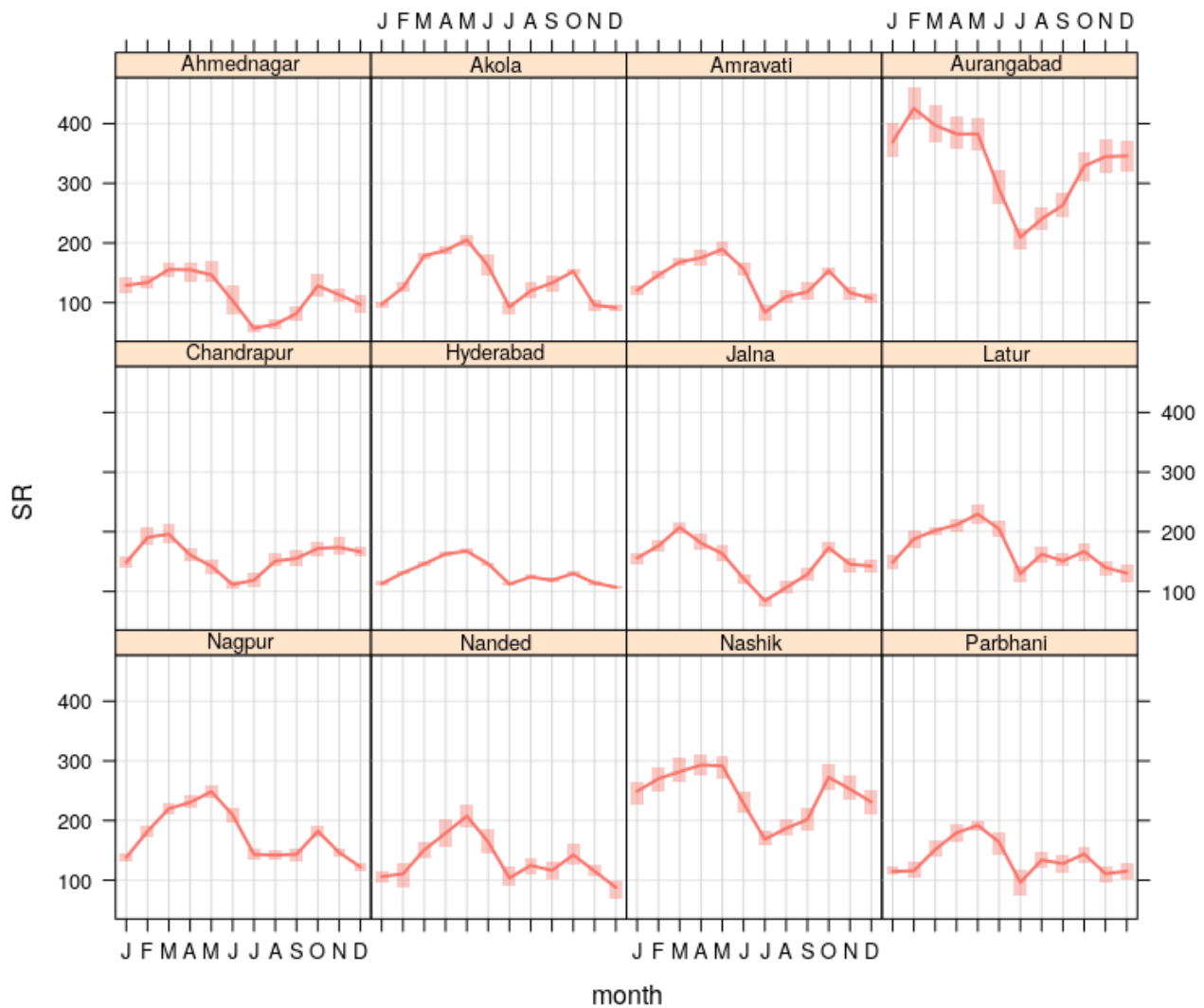
Figure 3 Monthly average solar radiation ( \text{W/m}^2 ) in the cities considered in the study (data source: CPCB)
