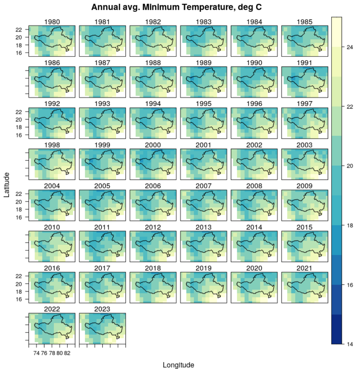
Figure 17 Annual average daily minimum temperature in the basin from 1980 to 2023
