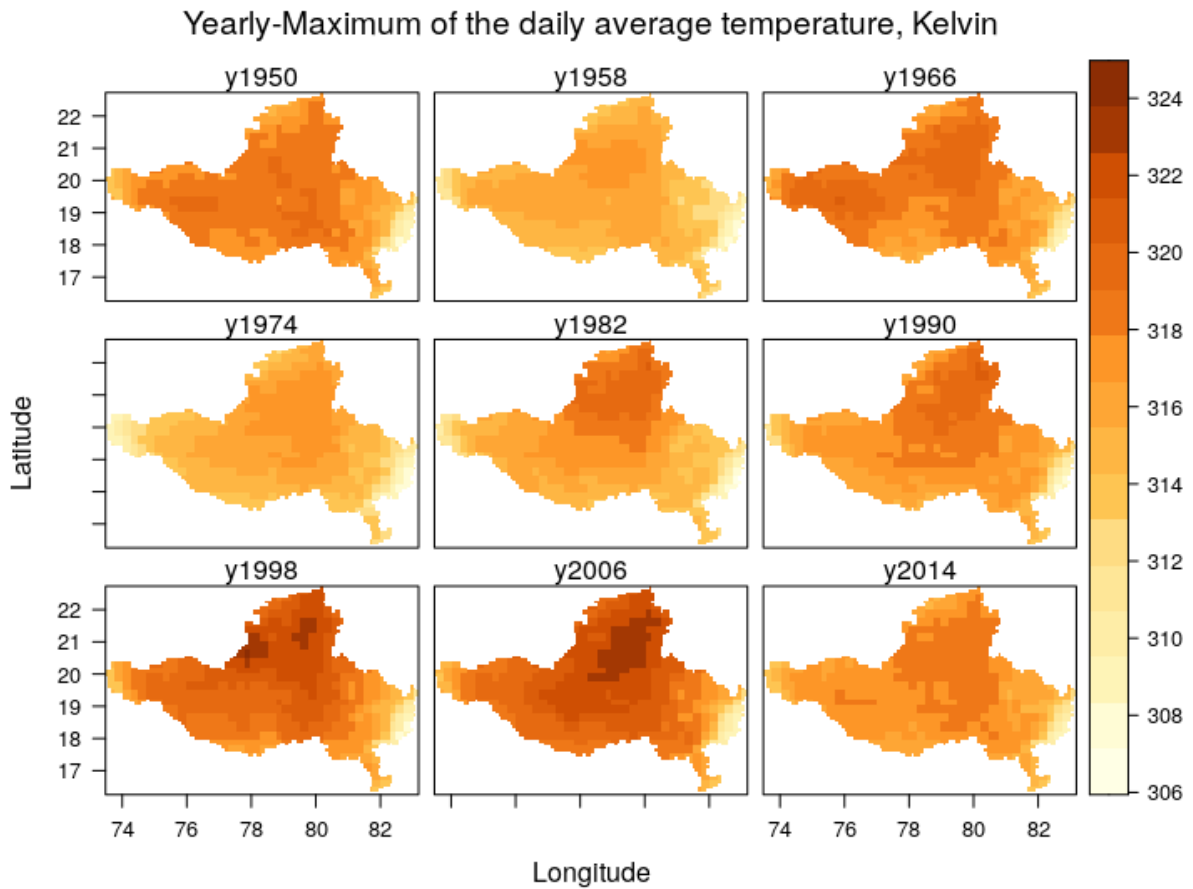
Figure 25 Yearly maximum of the daily-mean Temperature, K in the basin for several years during 1950-2014 (Source: NASA-GDDP-CMIP6). The values are simulation output of ACCESS-CM2 model
