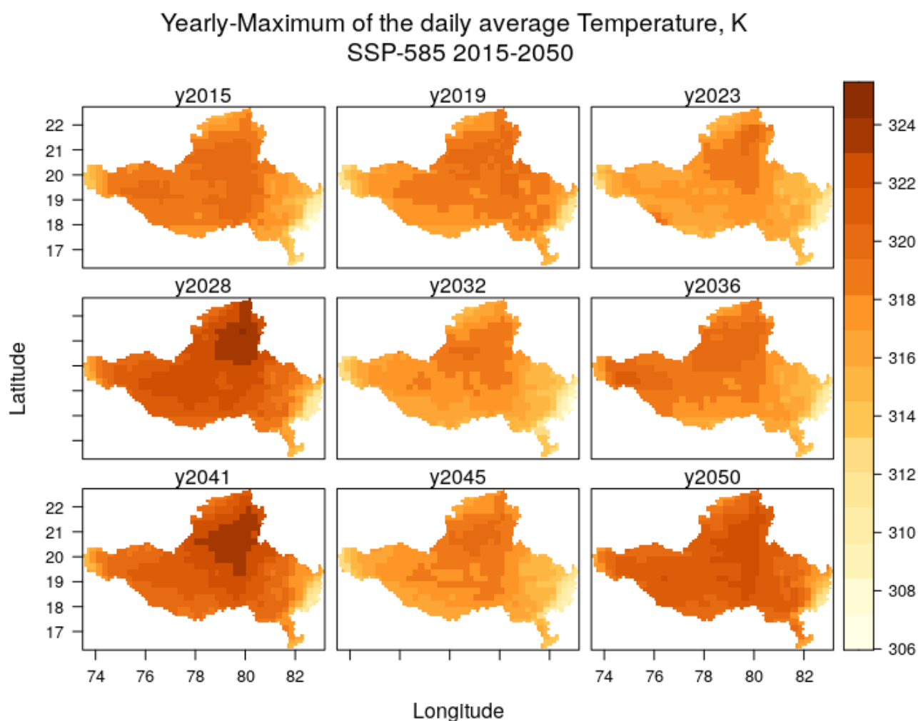
Figure 27 Yearly maximum of the daily-mean air temperature (K) in the basin for several years during 2015-2050 for the scenario SSP-585 (Source: NASA-GDDP-CMIP6). The values are simulation output of ACCESS-CM2 model
