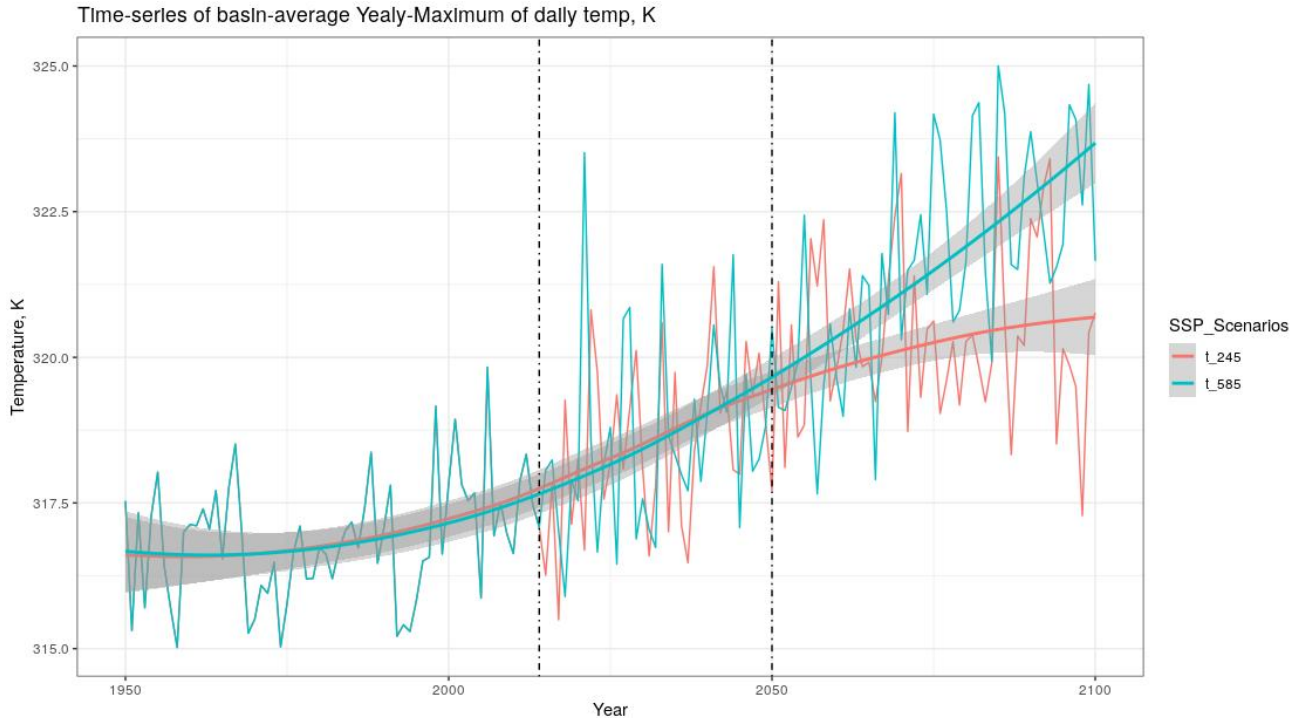
Figure 30 Time-series of basin-average of Yearly-maximum of daily temperature in Kelvins. The data ranges from 1950 to 2100 for future scenarios SSP-245 and SSP-585 from 2015
