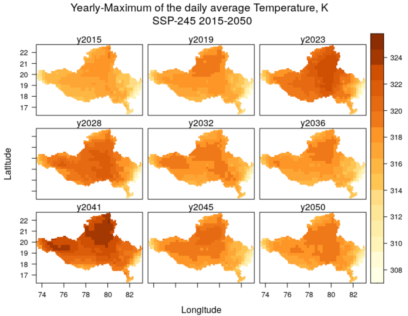
Figure 26 Yearly maximum of the daily-mean air temperature (K) in the basin for several years during 2015-2050 for the scenario SSP-245 (Source: NASA-GDDP-CMIP6). The values are simulation output of ACCESS-CM2 model
