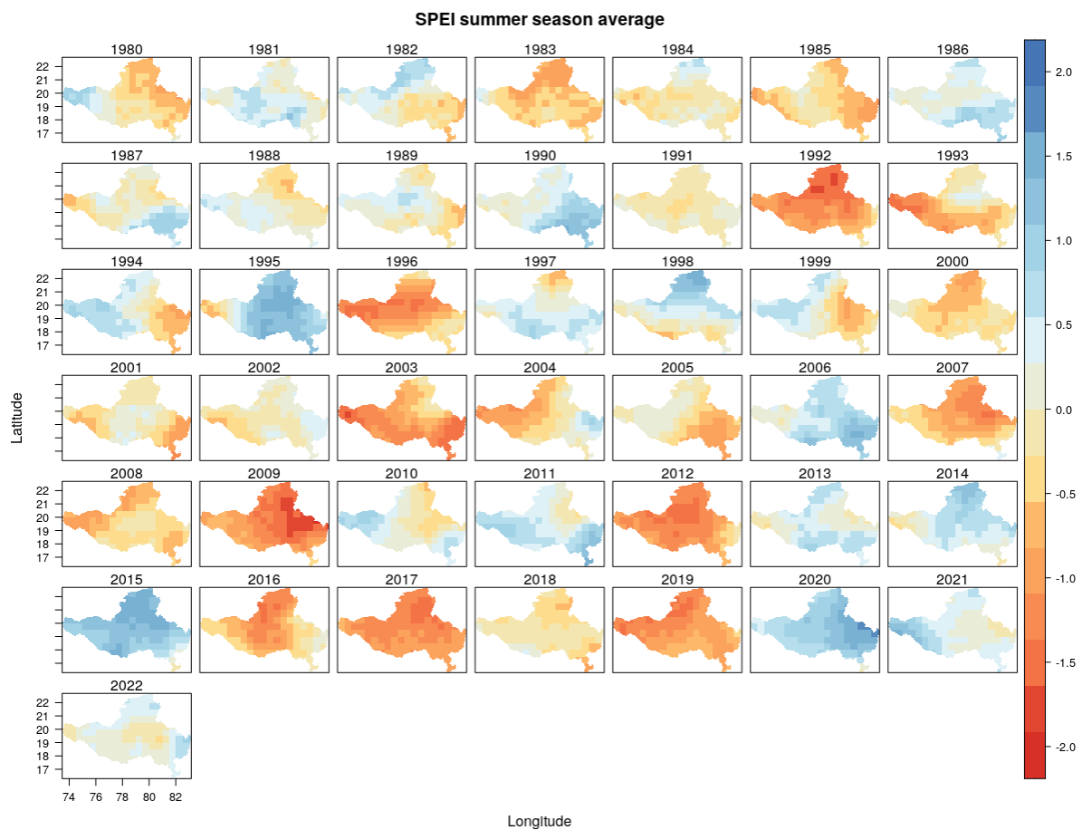
Figure 32 Summer season (MAMJ) average of SPEI values for years 1980 to 2023
