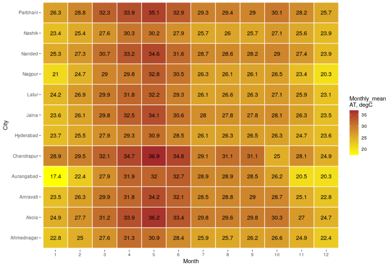
Figure 6 Heatmap of the Monthly average air temperature (°C) in the cities considered in the study (data source: CPCB)
