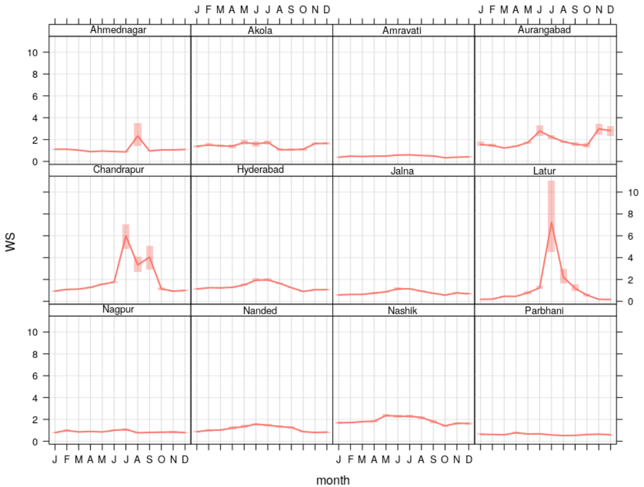
Figure 7 Monthly average wind speed (m/s) in the cities considered in the study (data source: CPCB)
