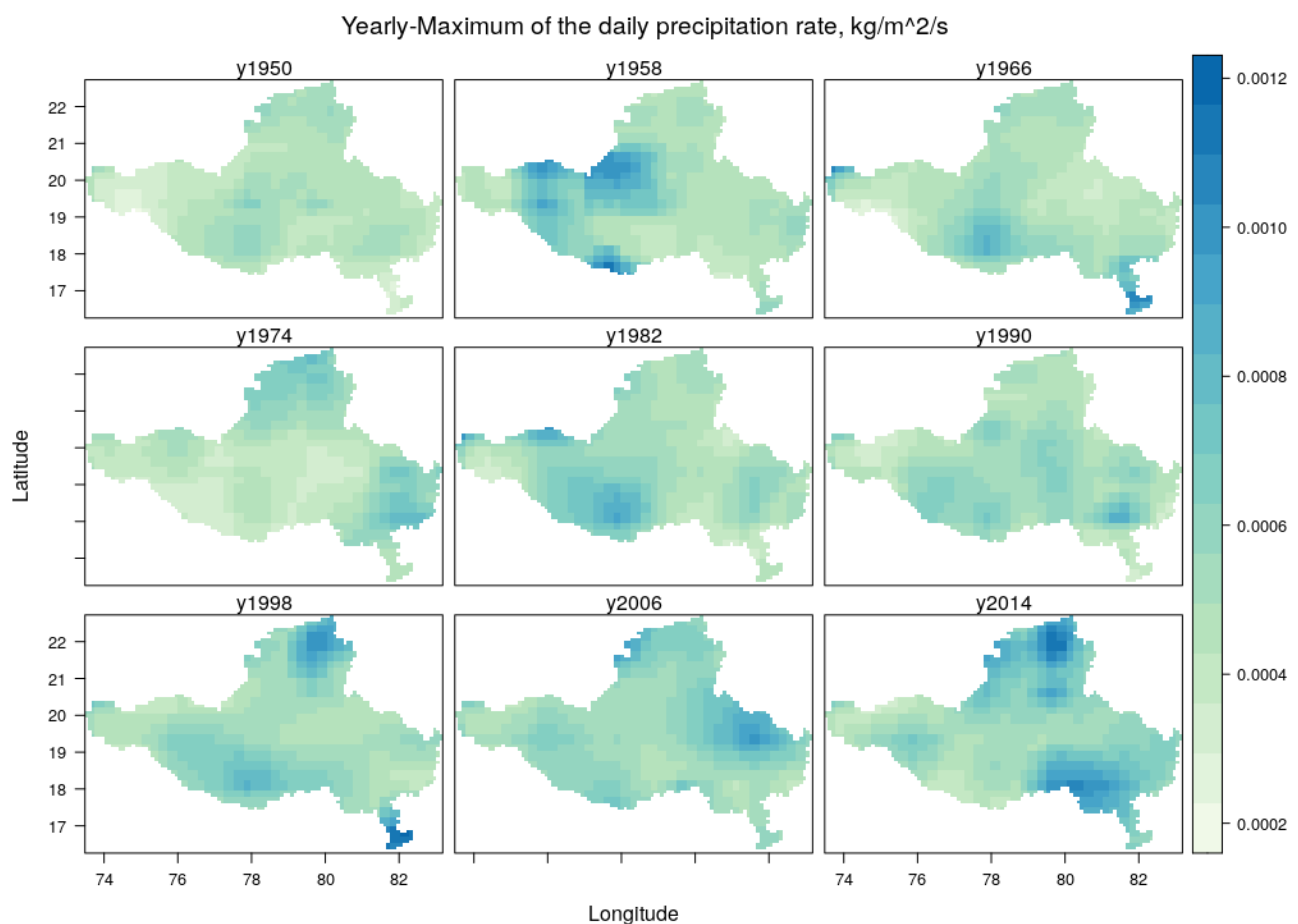
Figure 19 Yearly maximum of the daily-mean precipitation rate ( \text{kg/m}^2/\text{s} ) in the basin for several years during 1950-2014 (Source: NASA-GDDP-CMIP6). The values are simulation output of ACCESS-CM2 model
