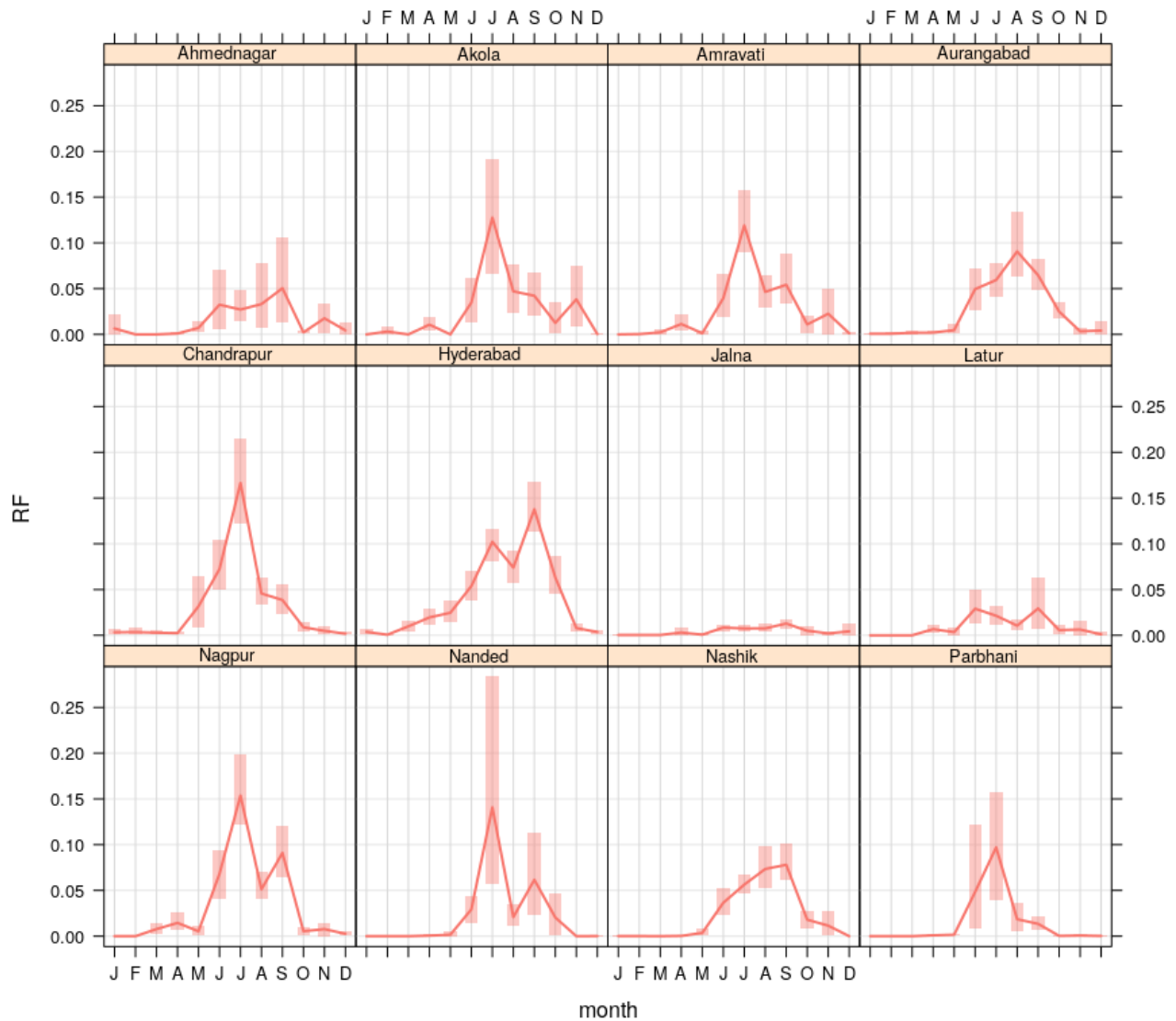
Figure 11 Monthly average Rainfall (mm) in the cities considered in the study (data source: CPCB)
