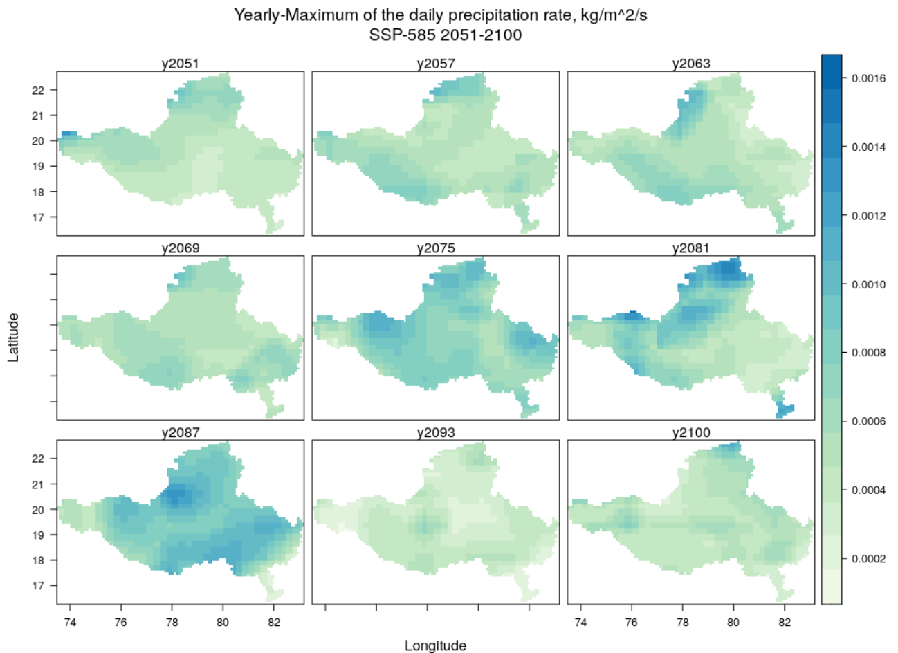
Figure 23 Yearly maximum of the daily-mean precipitation rate ( \text{kg/m}^2/\text{s} ) in the basin for several years during 2051-2100 for the scenario SSP-585 (Source: NASA-GDDP-CMIP6). The values are simulation output of ACCESS-CM2 model
