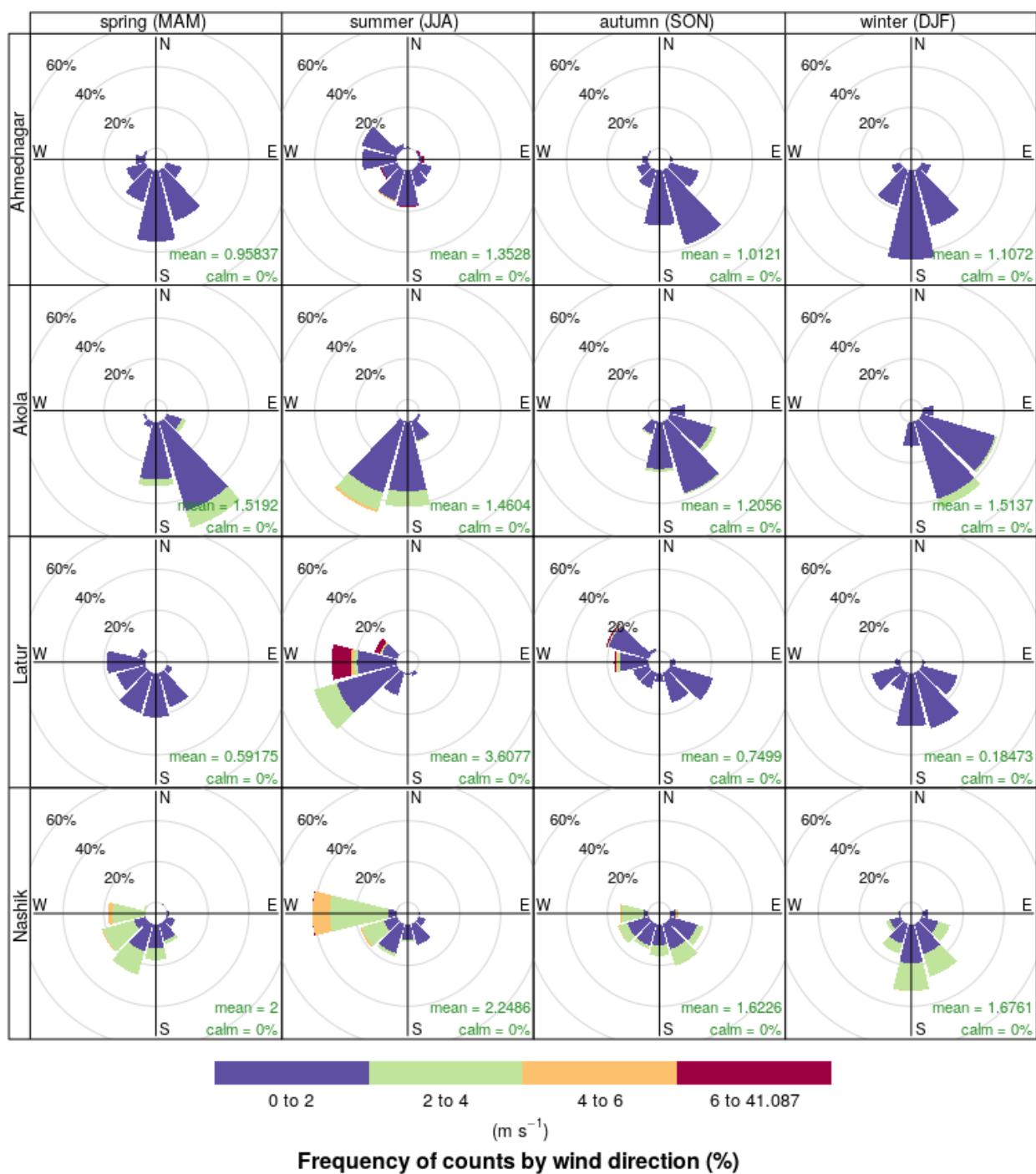
Figure 9 Monthly averaged windrose diagram for Ahmednagar, Akola, Latur, and Nashik cities (Source: CPCB)
