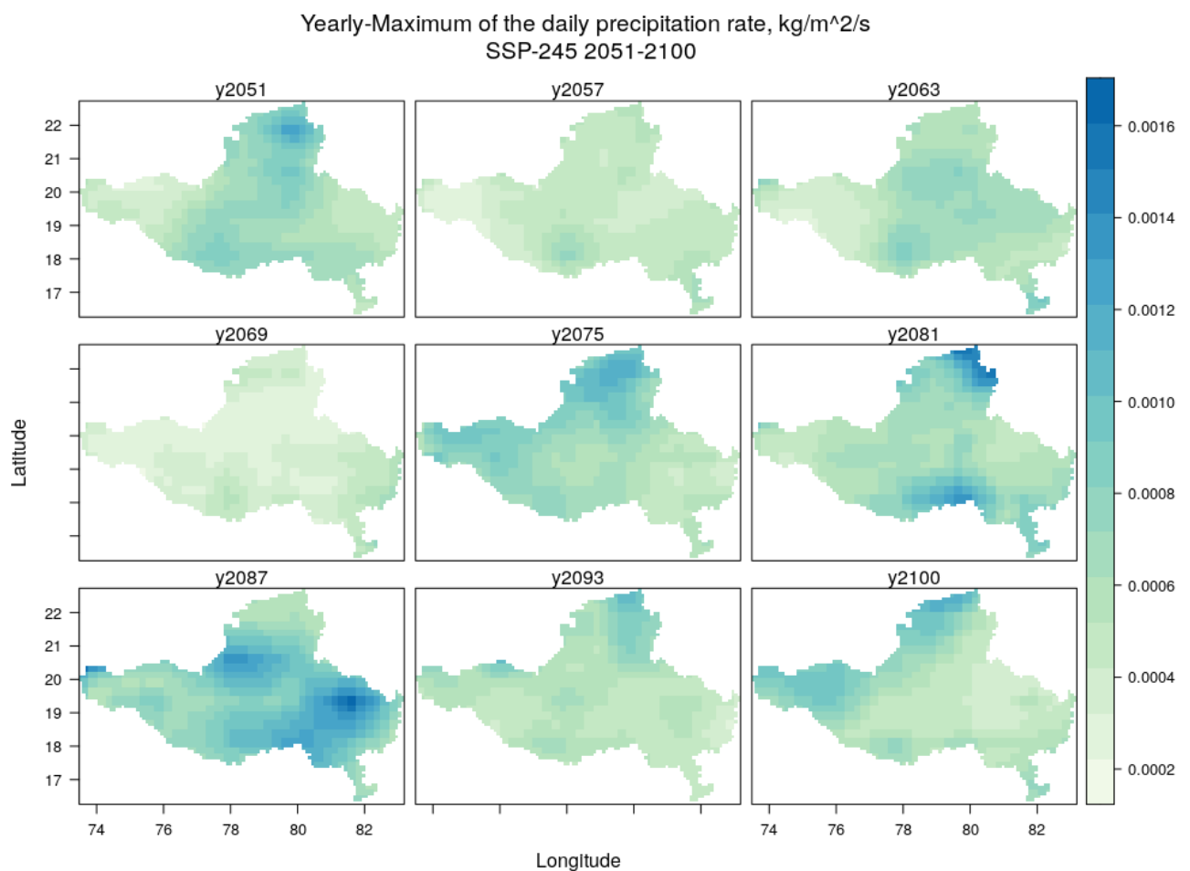
Figure 22 Yearly maximum of the daily-mean precipitation rate (kg/m 2 /s) in the basin for several years during 2051-2100 for the scenario SSP-245 (Source: NASA-GDDP-CMIP6). The values are simulation output of ACCESS-CM2 model
