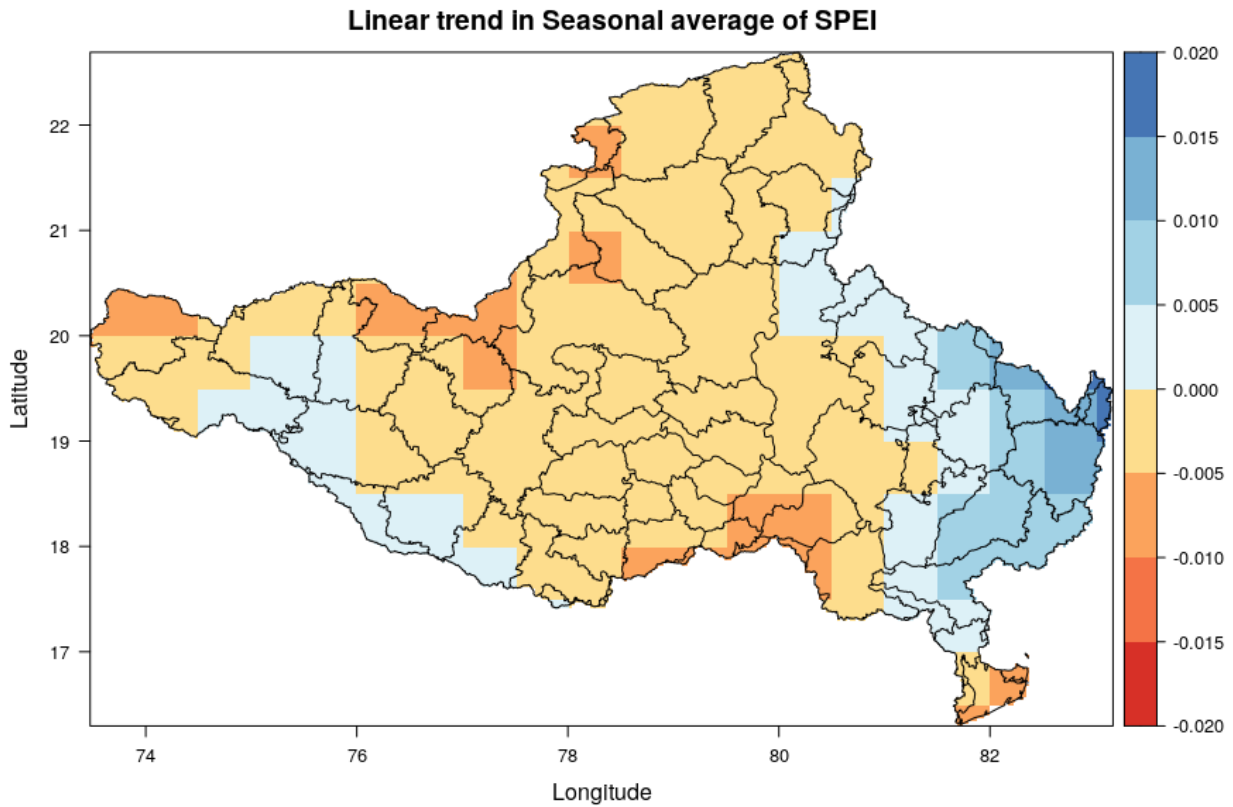
Figure 33 Linear trend in the SPEI values for summer season (MAMJ)
