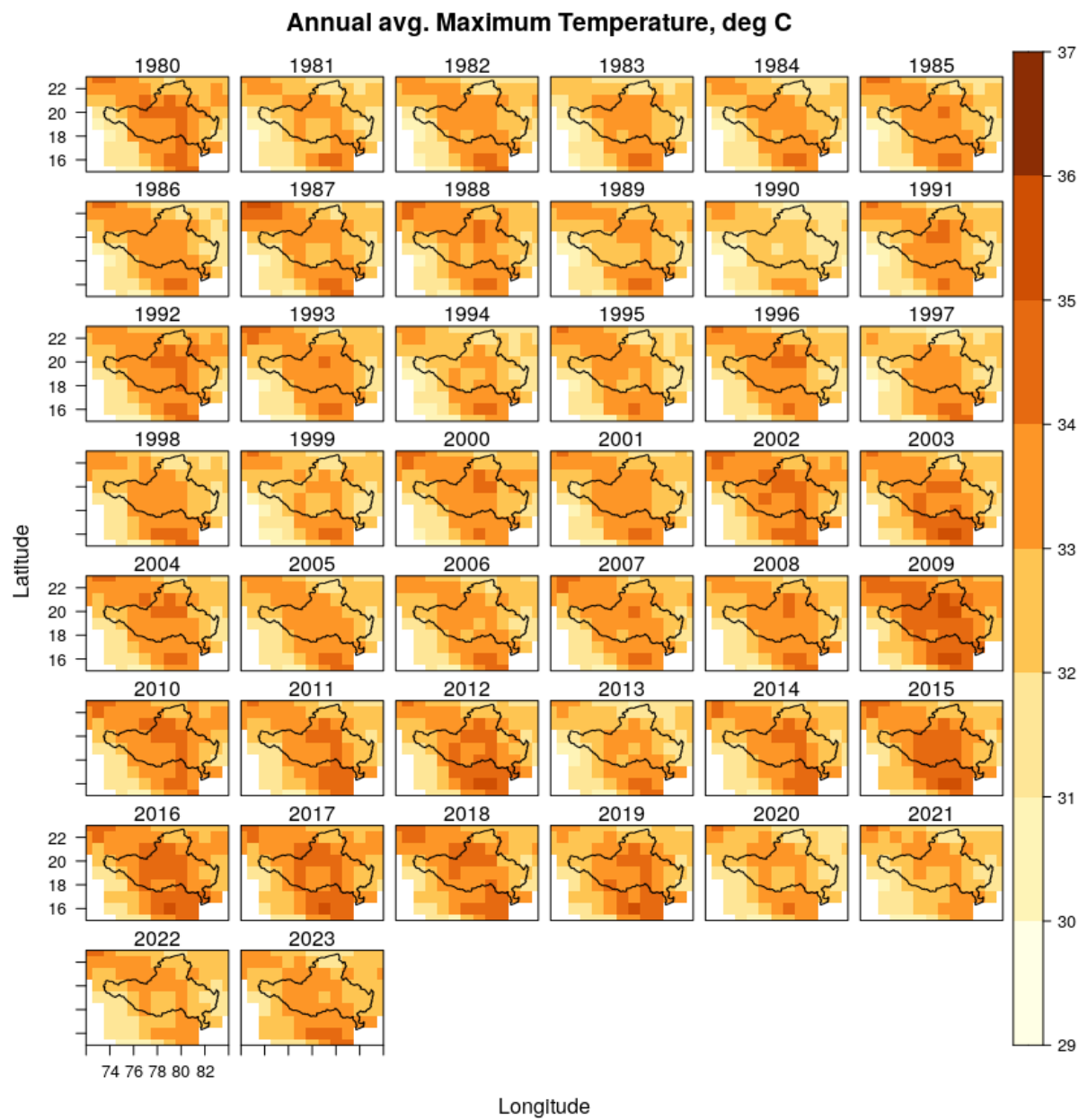
Figure 15 Annual average daily maximum temperature in the basin from 1980 to 2023
