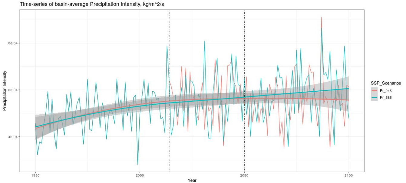
Figure 24 Time-series of the basin-average precipitation intensity ( \text{kg/m}^2/\text{s} ) from 1950 to 2100 for two different SSP scenarios SSP-245 and SSP-585 from 2015
