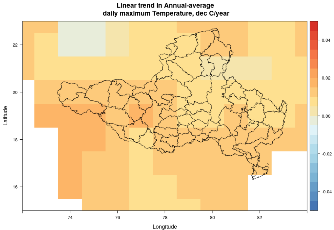
Figure 16 Temporal gradient of annual average daily maximum temperature ( ^{\circ}\text{C}/\text{year} ) in the basin during 1980 to 2023
