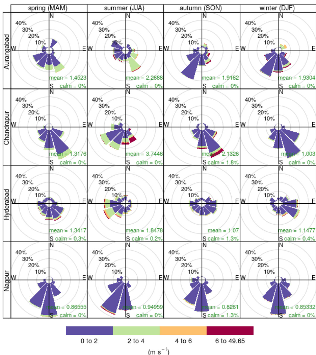
Figure 8 Monthly averaged windrose diagram for Aurangabad, Chandrapur, Hyderabad, and Nagpur cities (Source: CPCB)
