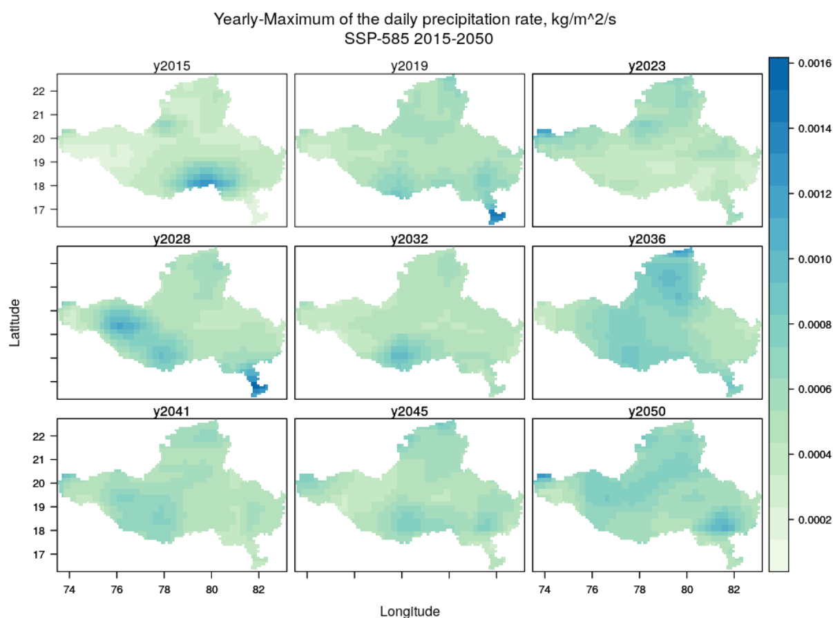
Figure 21 Yearly maximum of the daily-mean precipitation rate ( \text{kg/m}^2/\text{s} ) in the basin for several years during 2015-2050 for the scenario SSP-585 (Source: NASA-GDDP-CMIP6). The values are simulation output of ACCESS-CM2 model
