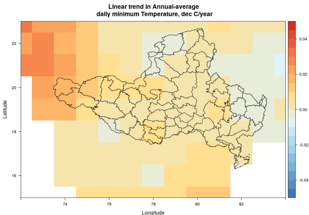
Figure 18 Temporal gradient of annual average daily minimum temperature ( ^{\circ}\text{C}/\text{year} ) in the basin during 1980 to 2023
