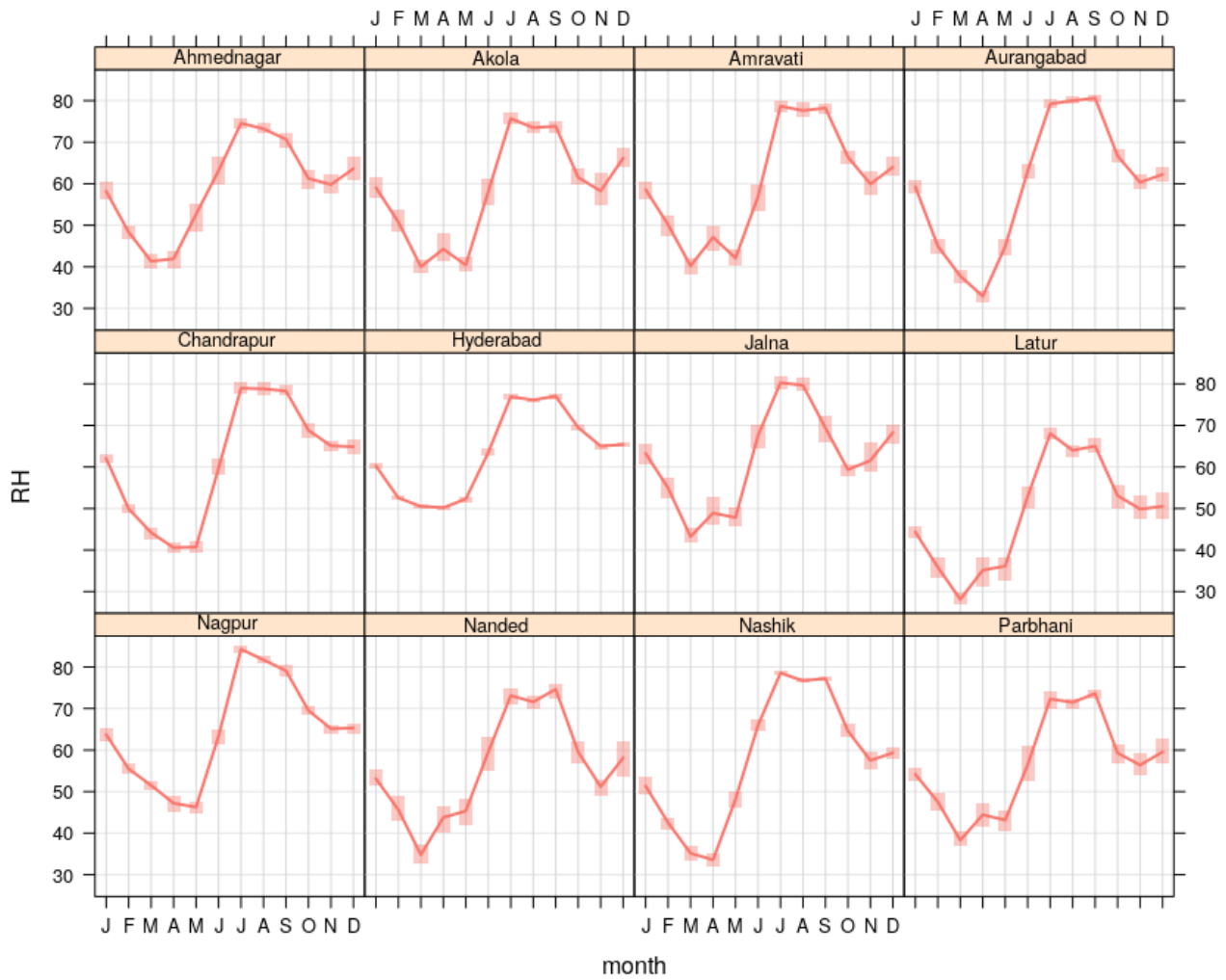
Figure 12 Monthly average Relative Humidity (%) in the cities considered in the study (data source: CPCB)
