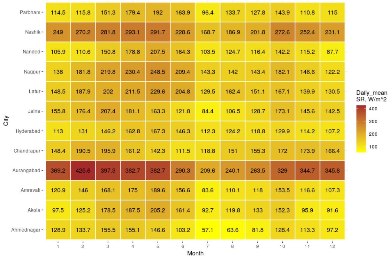
Figure 4 Heatmap of the Monthly average solar radiation (W/m 2 ) in the cities considered in the study (data source: CPCB)
