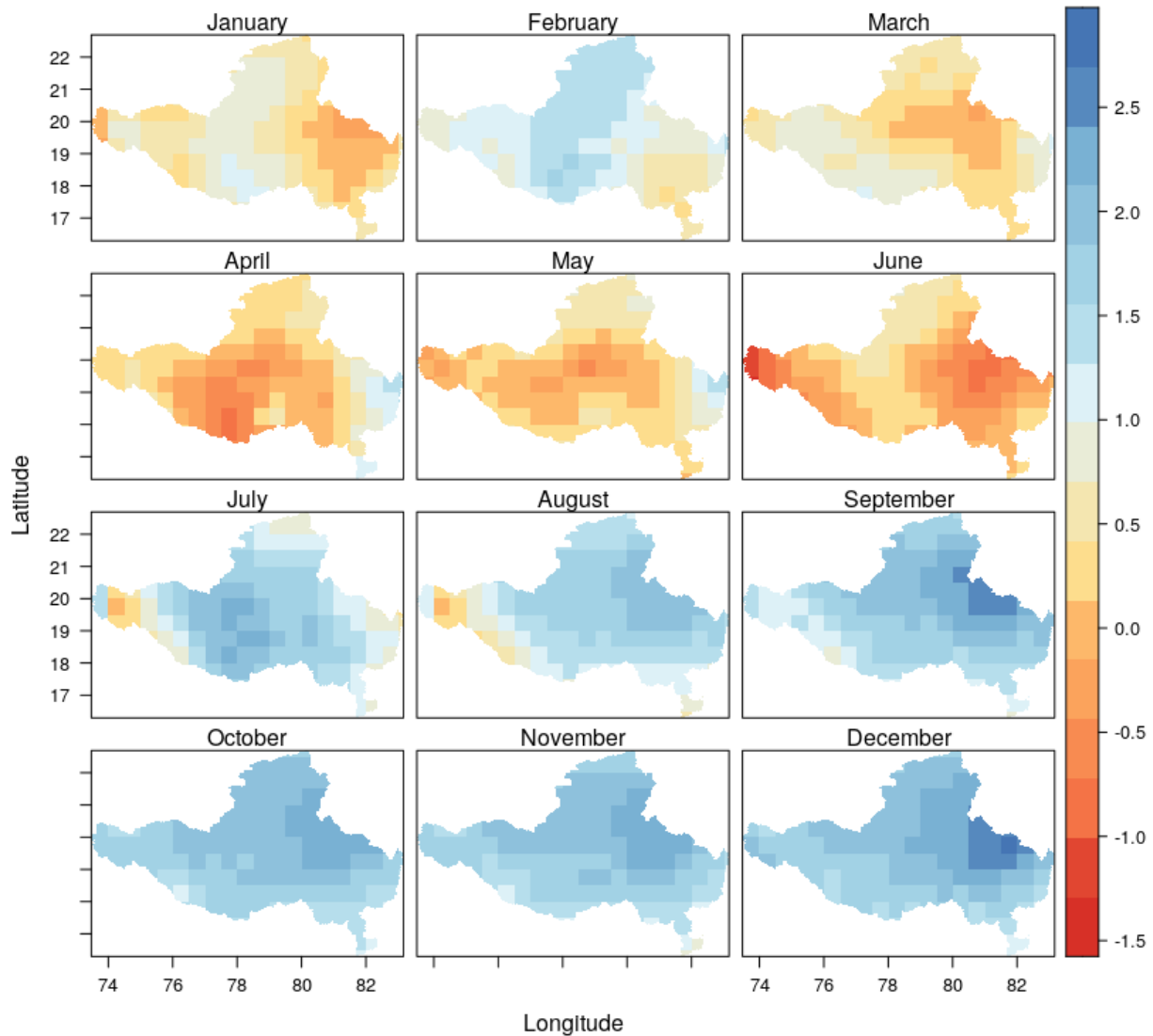
Figure 31 Monthly average SPEI values in Godavari Basin for 2022. Source: CSIC-SPEI
