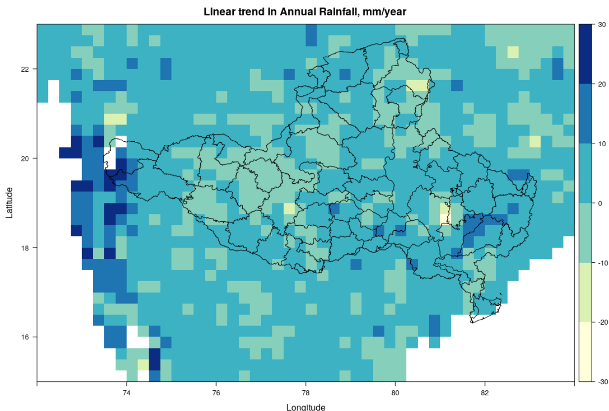
Figure 14 Temporal gradient of annual precipitation (mm/year) in the basin during 1980 to 2023
