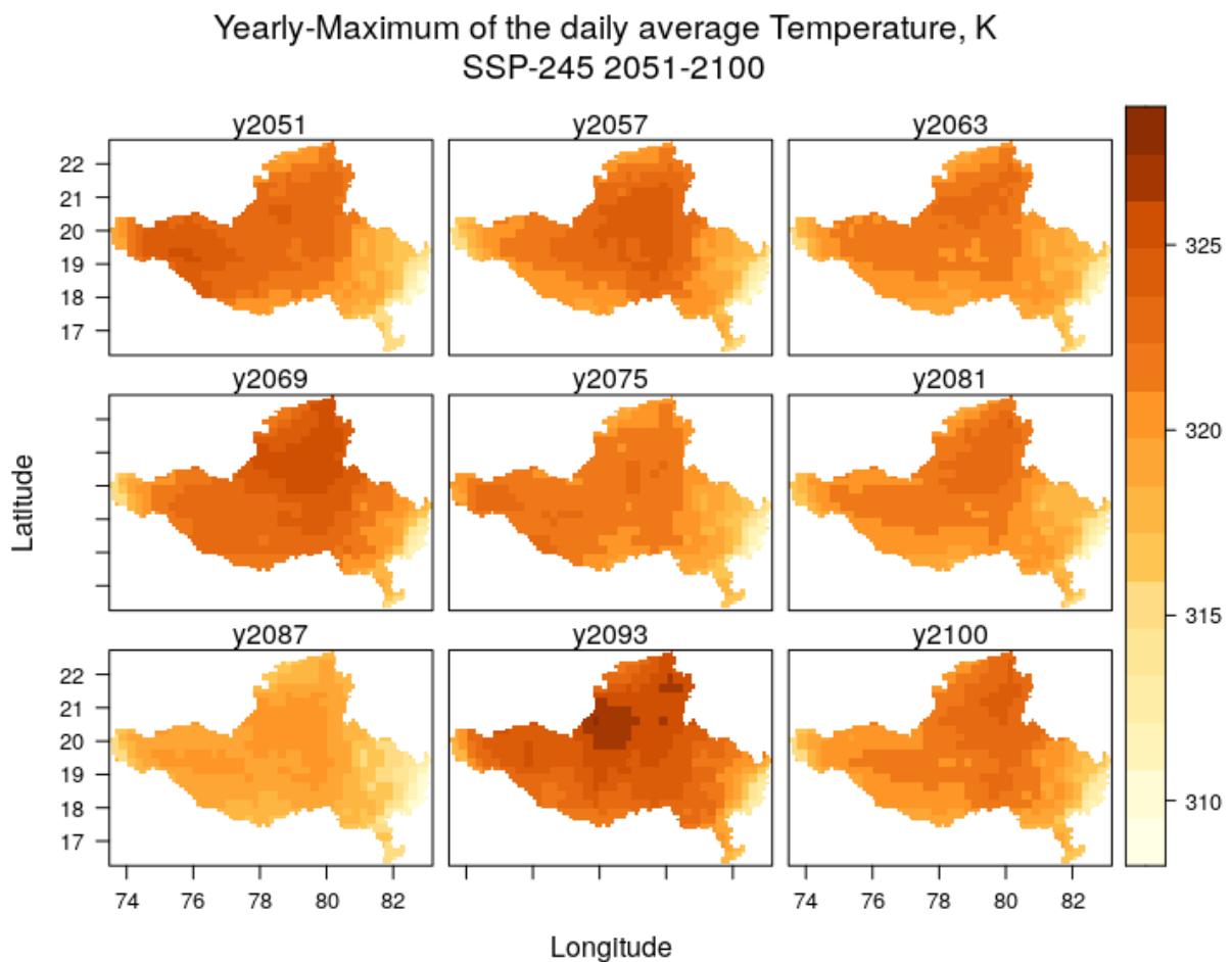
Figure 28 Yearly maximum of the daily-mean air temperature (K) in the basin for several years during 2051-2100 for the scenario SSP-245 (Source: NASA-GDDP-CMIP6). The values are simulation output of ACCESS-CM2 model
