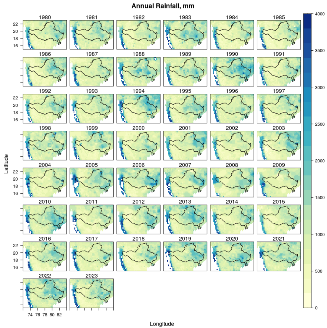
Figure 13 Annual rainfall in the basin from 1980 to 2023
