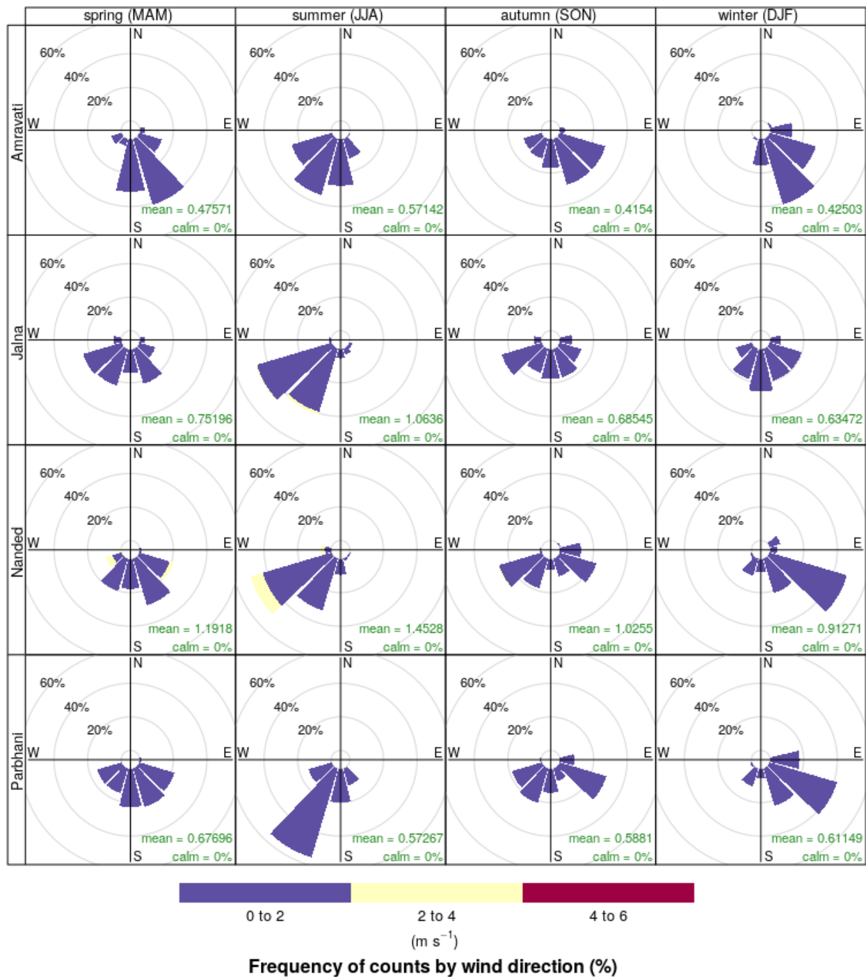
Figure 10 Monthly averaged windrose diagram for Amravati, Jalna, Nanded, and Parbhani cities (Source: CPCB)
