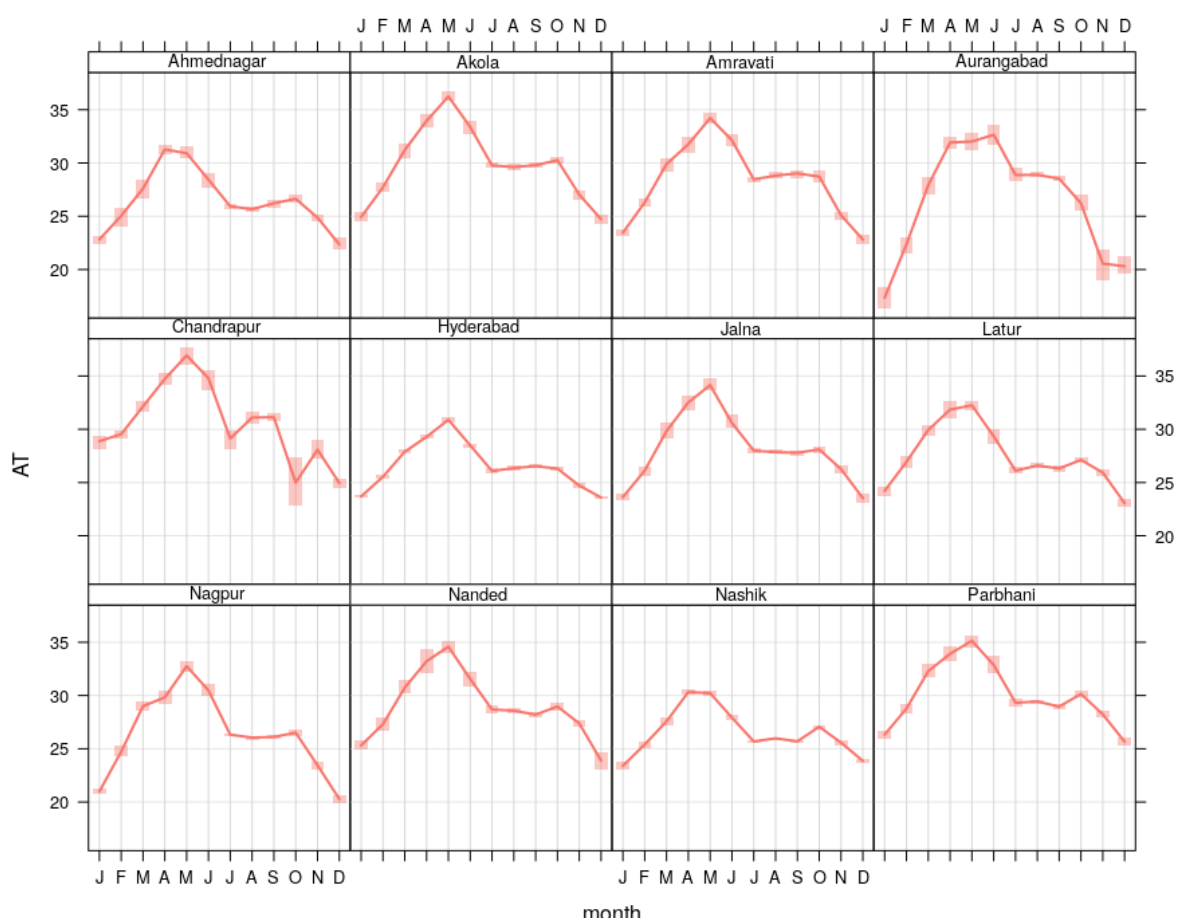
Figure 5 Monthly average air temperature (AT, in deg C) in the cities considered in the study (data source: CPCB)
