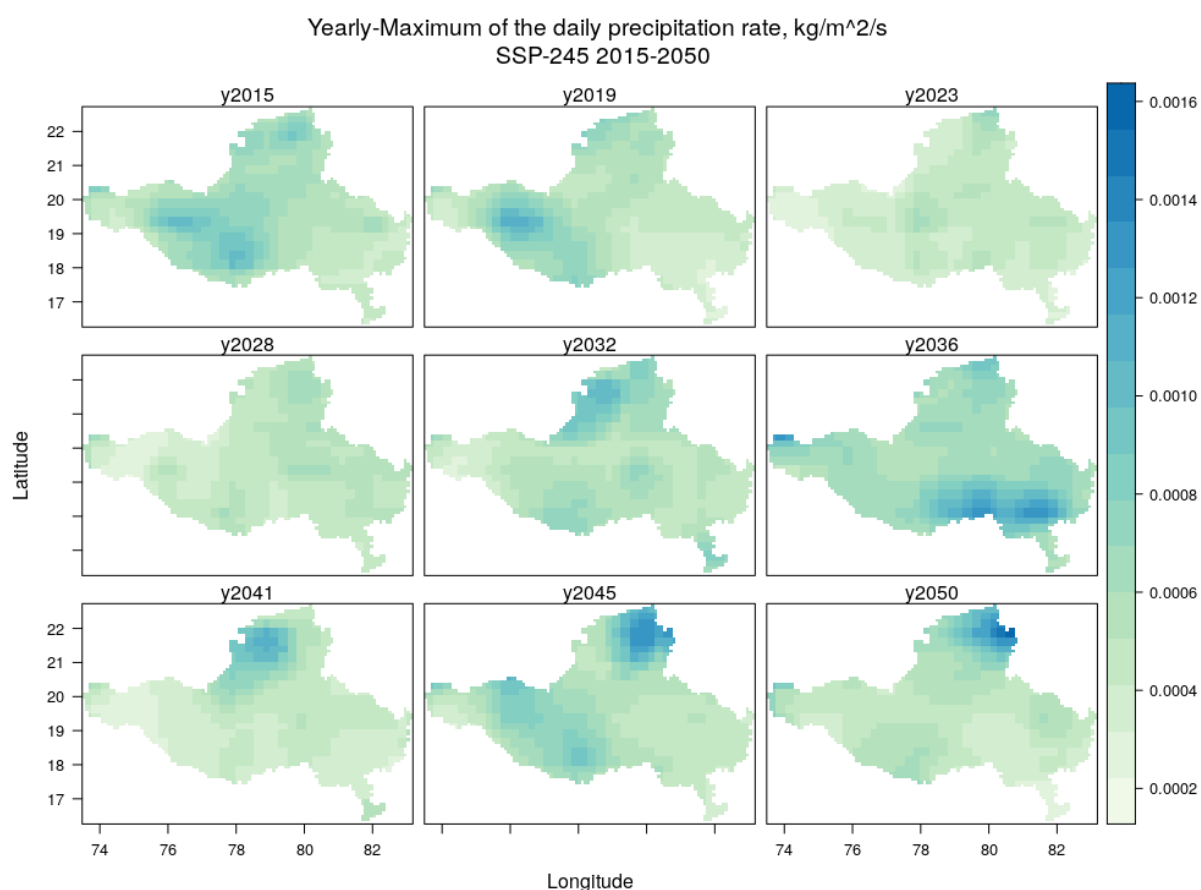
Figure 20 Yearly maximum of the daily-mean precipitation rate ( \text{kg/m}^2/\text{s} ) in the basin for several years during 2015-2050 for the scenario SSP-245 (Source: NASA-GDDP-CMIP6). The values are simulation output of ACCESS-CM2 model
