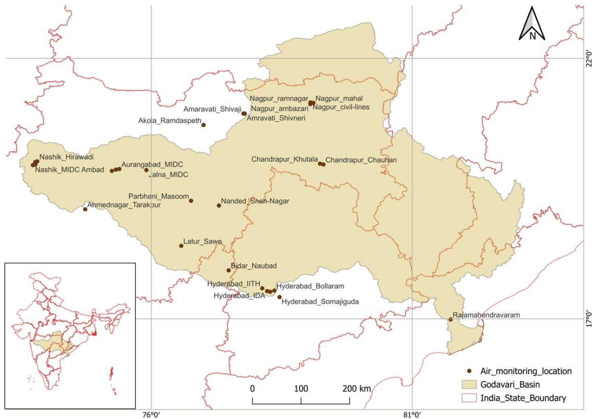
Figure 2 Location of CPCB monitoring sites in the basin
