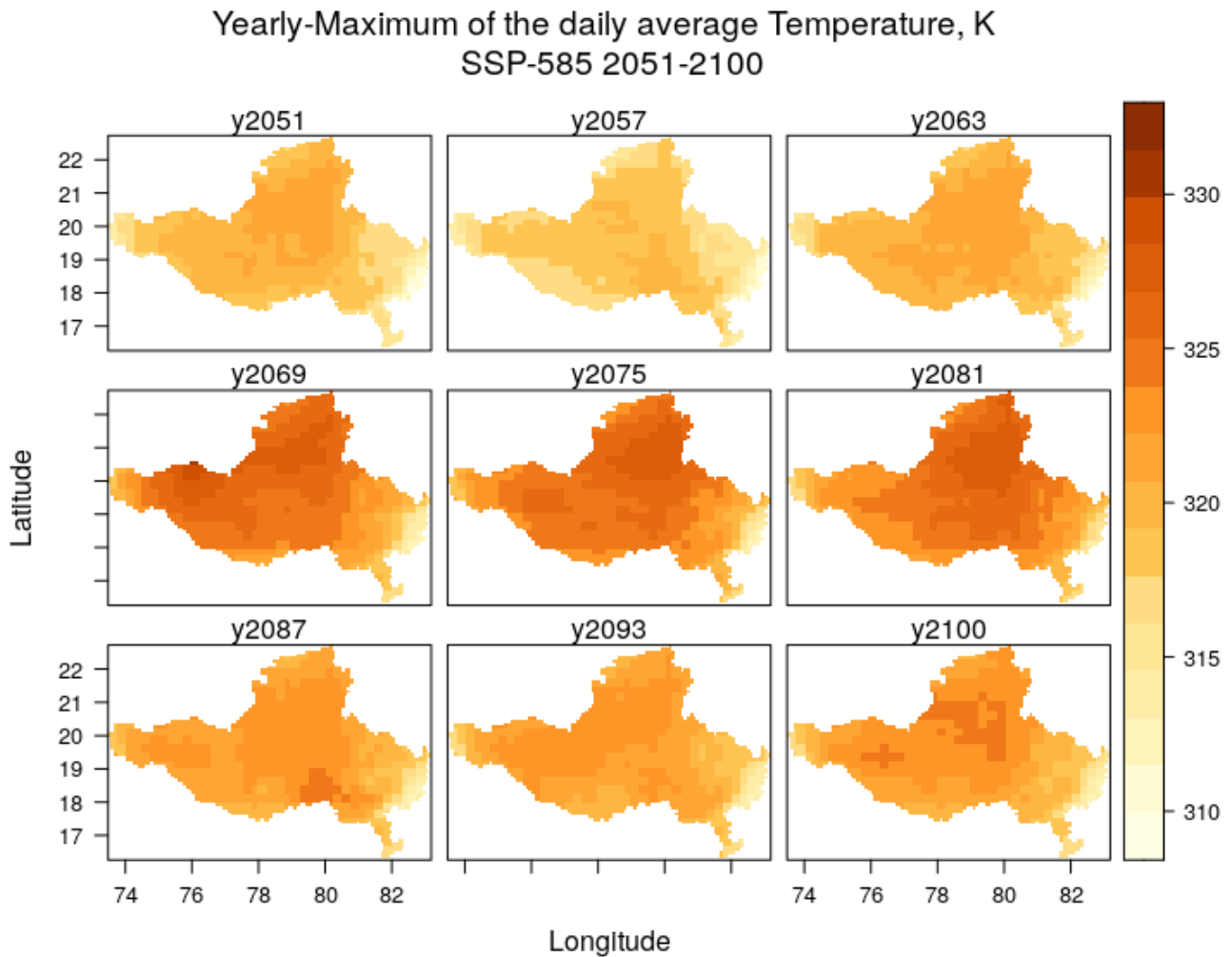
Figure 29 Yearly maximum of the daily-mean air temperature (K) in the basin for several years during 2051-2100 for the scenario SSP-585 (Source: NASA-GDDP-CMIP6). The values are simulation output of ACCESS-CM2 model
